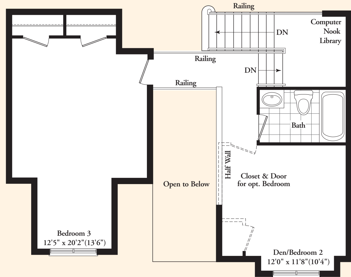
LOFT FLOOR PLAN
